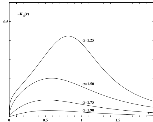
Fig. 1b – Plots of the basic spectral function -K_\alpha(r) for 1 < \alpha < 2
