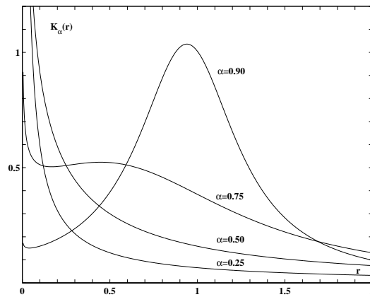
Fig. 1a – Plots of the basic spectral function K_\alpha(r) for 0 < \alpha < 1
