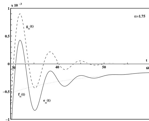
Fig. 3c – Decay of the basic fundamental solution u_0(t) = e_\alpha(t) for \alpha = 1.75
