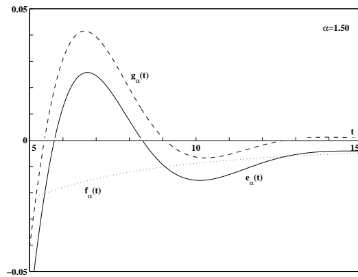
Fig. 3b – Decay of the basic fundamental solution u_0(t) = e_\alpha(t) for \alpha = 1.50
