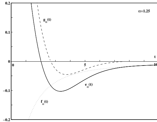
Fig. 3a – Decay of the basic fundamental solution u_0(t) = e_\alpha(t) for \alpha = 1.25
